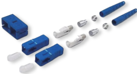
SC/PC/SM/DX3.0(SC30-2113141) Component drawing
