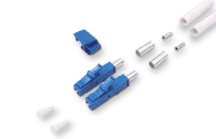
DLC/PC/SM/DX3.0(DLC30-113161) Exploded views
